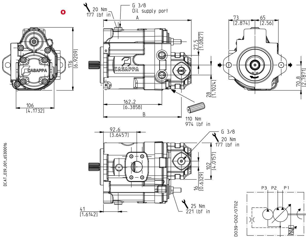
KAPPA gear units
