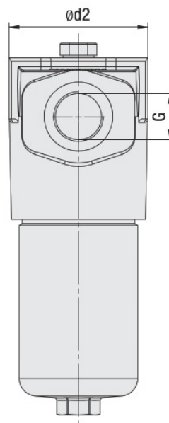
Threaded connection
