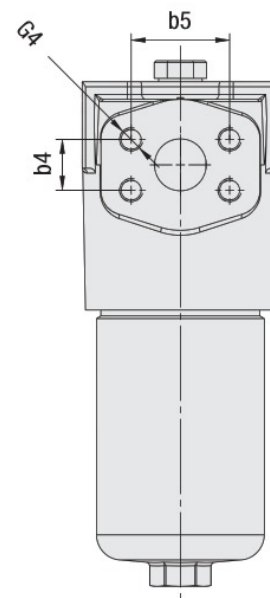
Flange connection
